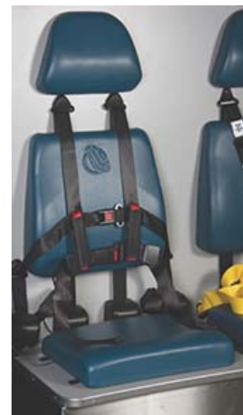
1506 6-Point Belt system
